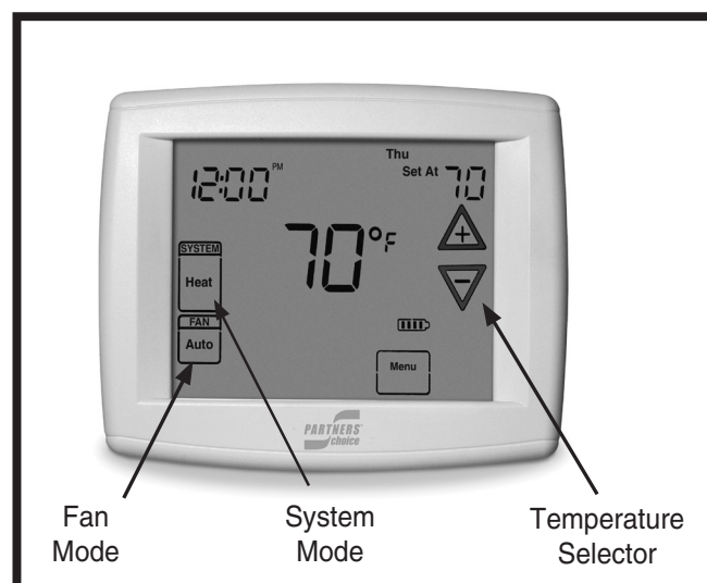
Figure 1. Digital Thermostat
